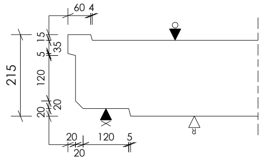
DETAIL 2 1:10
