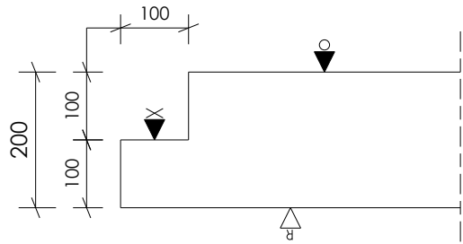
DETAIL 1 1:10
